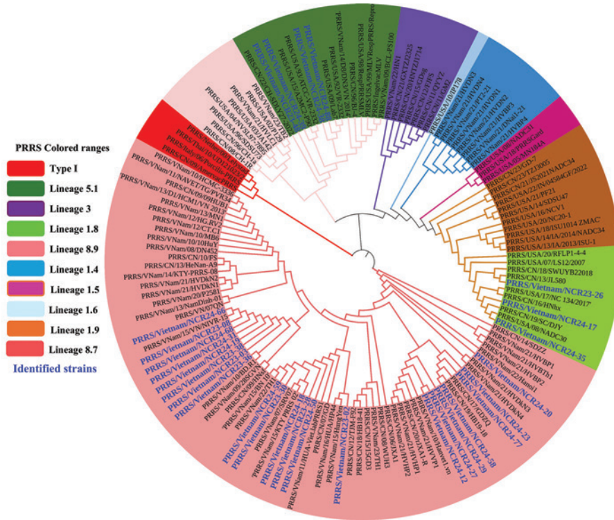
Figure 1. Phylogenetic analysis based on the ORF5 protein sequences. PRRSV strains identified in this study are shown in blue bold, and reference PRRSV strains are shown in black. The phylogenetic tree was constructed using the neighbor-joining method in MEGA software with 1,000 bootstrap replicates.
